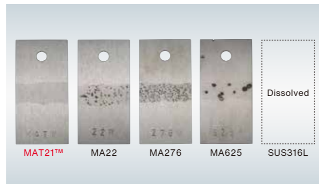
Example of pitting corrosion resistance test results for Proterial's corrosion-resistant material 24 hours at boiling temperature (104° C) in 11.5% H 2 SO 4 + 1.2% HCl + 1% FeCl 3 + 1% CuCl 2
